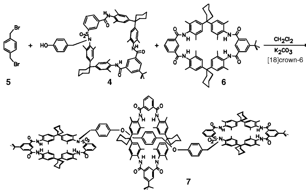
Scheme 4. Divergent synthesis of a rotaxane assembly in the generation zero.
