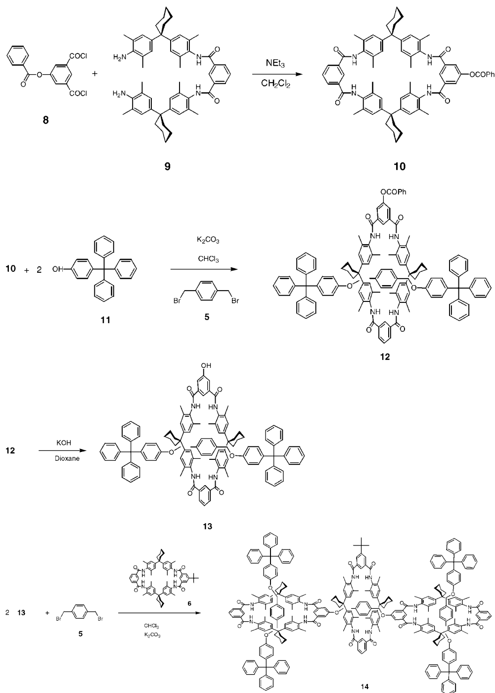
Scheme 5. Convergent synthesis of a dendritic rotaxane assembly 14 of generation one.
