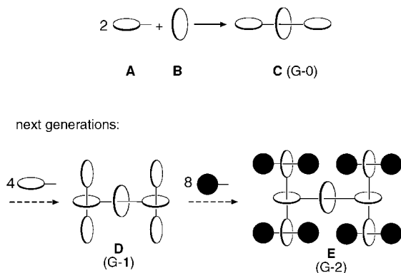
Scheme 1. General concept for the divergent synthesis of rotaxane assemblies of increasing generation (G).
