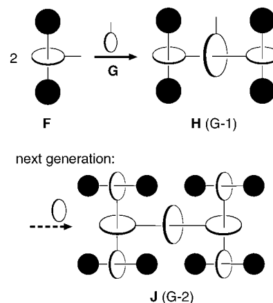
Scheme 2. Convergent synthesis of rotaxane assemblies.
