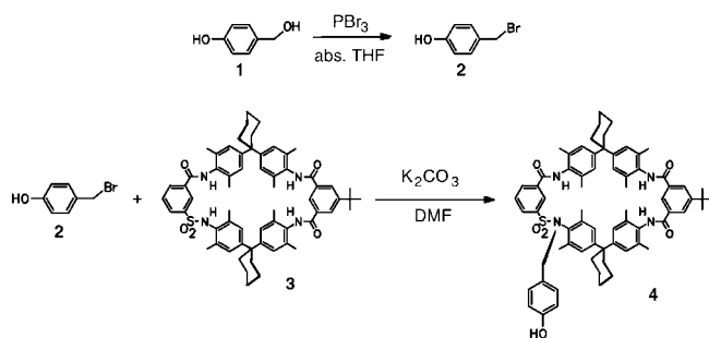
Scheme 3. Synthesis of the wheel acting as stopper.
