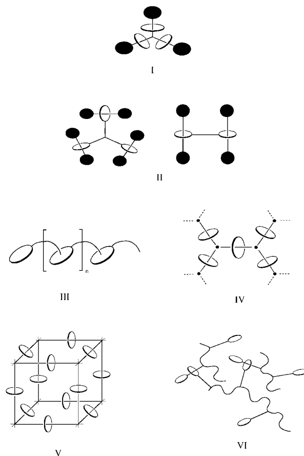
Figure 1. Known rotaxane assemblies; I: axle-linked assembly; II: wheel-linked assembly; III: linear one-dimensional oligorotaxane; IV: two-dimensional polyrotaxane; V: three-dimensional polyrotaxane; VI: rotaxane network.
